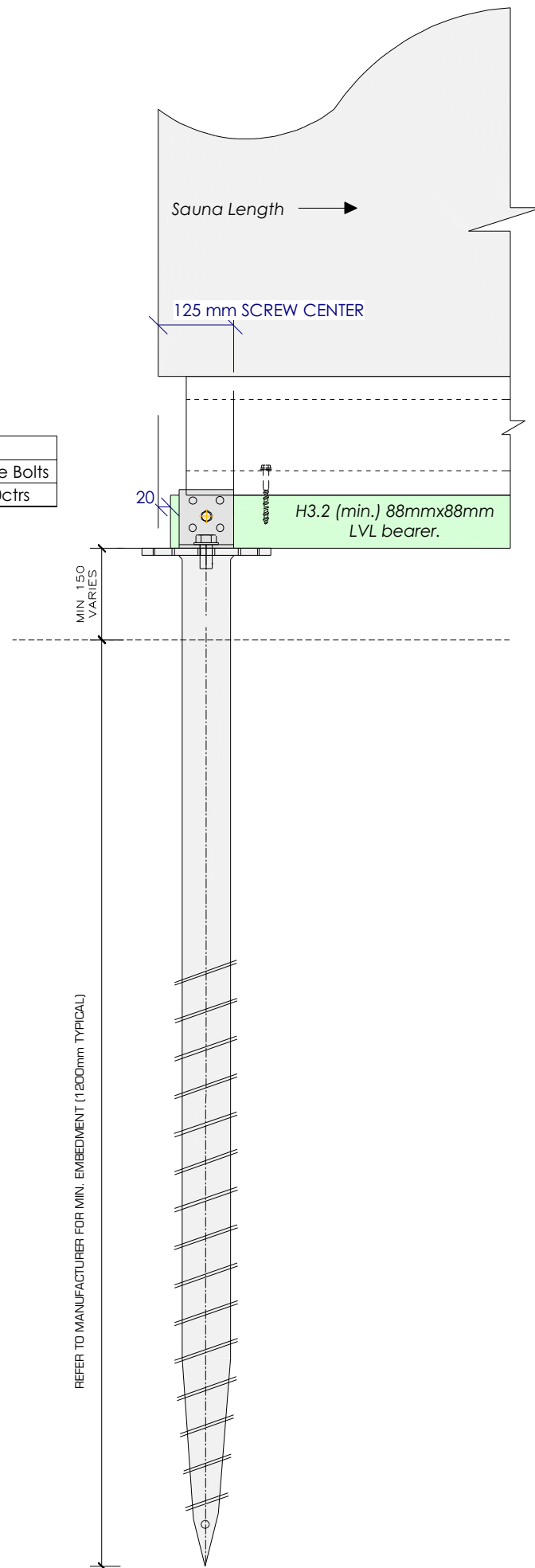
Cross Section A/A scale 1:10
