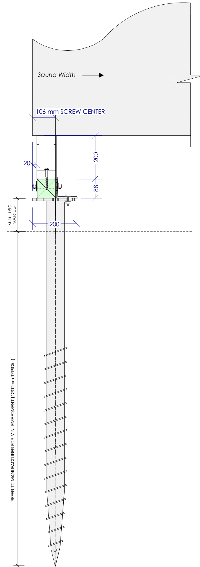
Cross Section B/B scale 1:10
